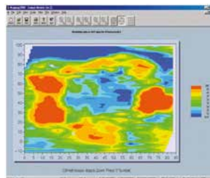
Map of OhmMapper Resistivity Data
