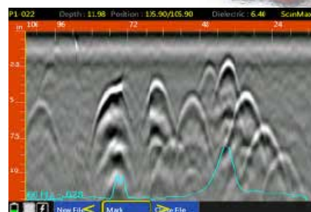
Screen image illustrates GPR data of a suspended concrete slab with metallic reinforcement and a conduit with the presence of live power, indicated by the blue peaks.
